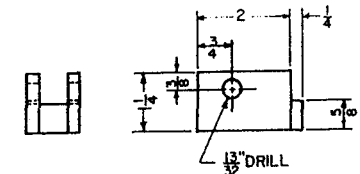
HINGE DETAILS
