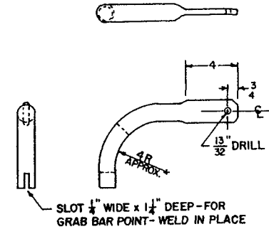
GRAB BAR DETAILS
